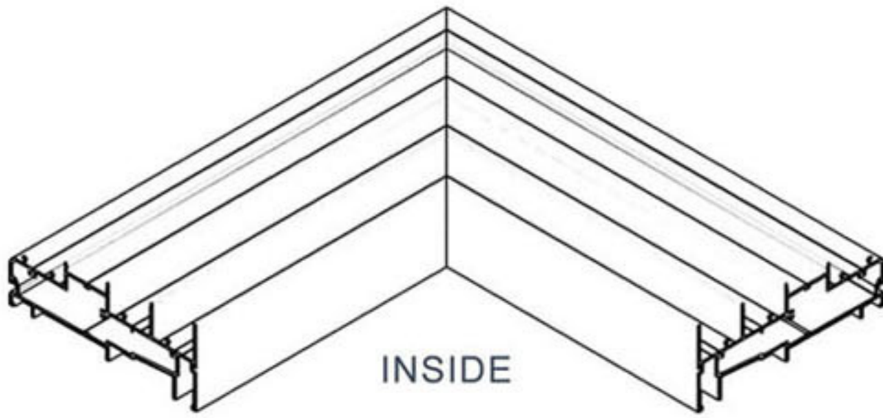
Multi Track Sill - External Corner
